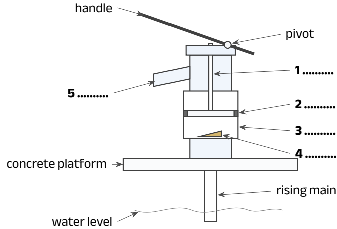
Figure 12.2: The Village Hand Pump
